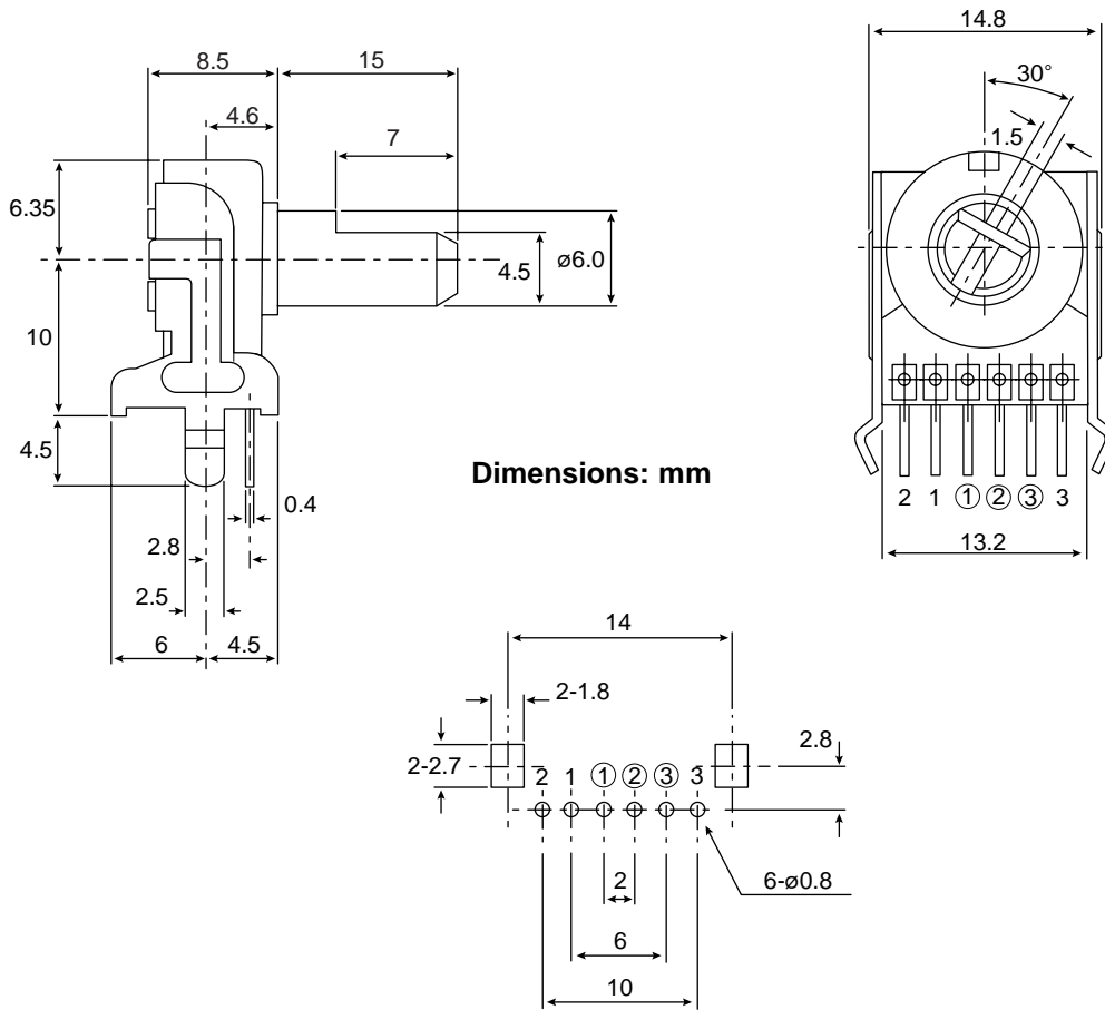
P.C.B. Mounting Hole Detail
