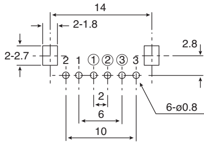
P.C.B. Mounting Hole Detail
