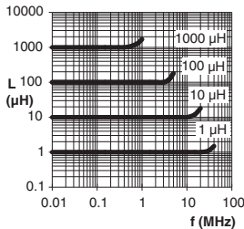
Typical L vs Frequency(f)
