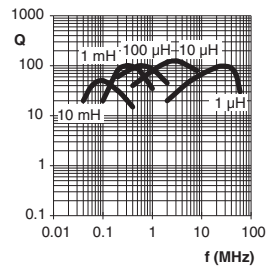
Typical Q vs Frequency(f)
