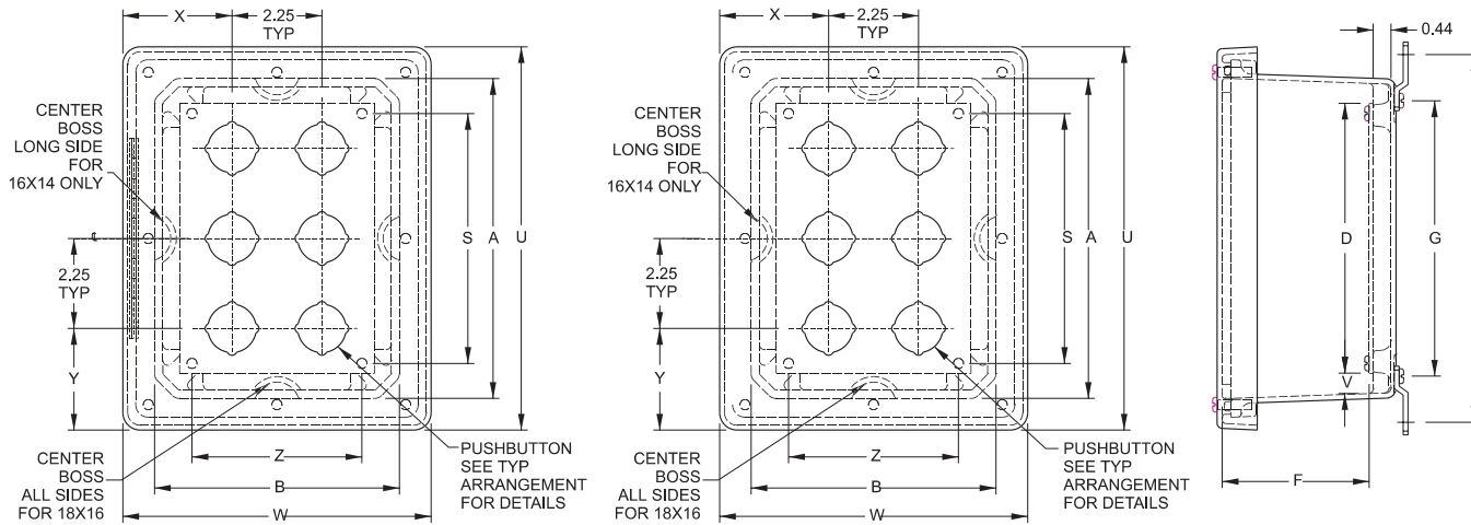
Top View Hinged Screw Cover
