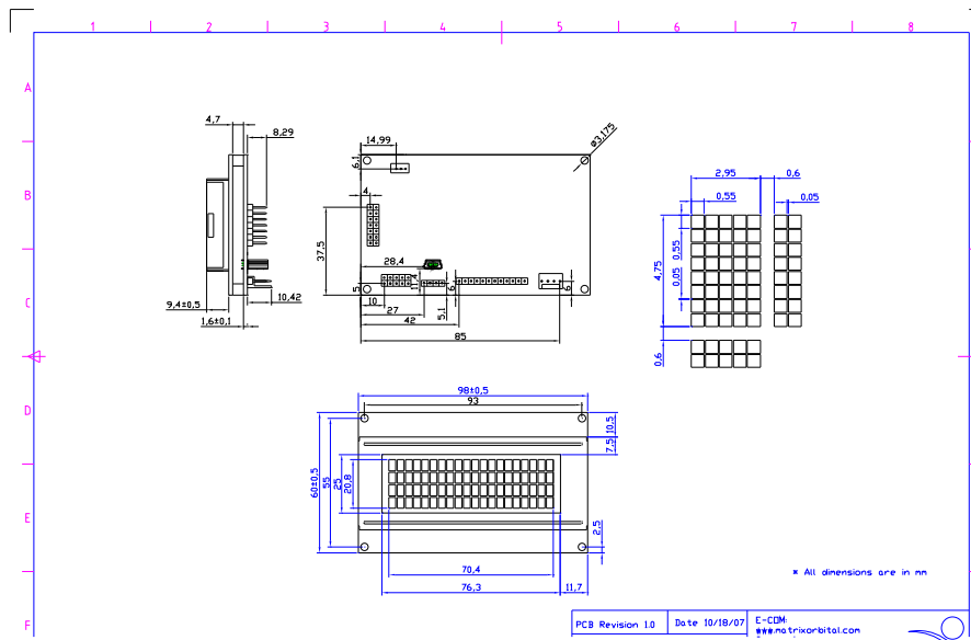
Figure 17: Physical Diagram
