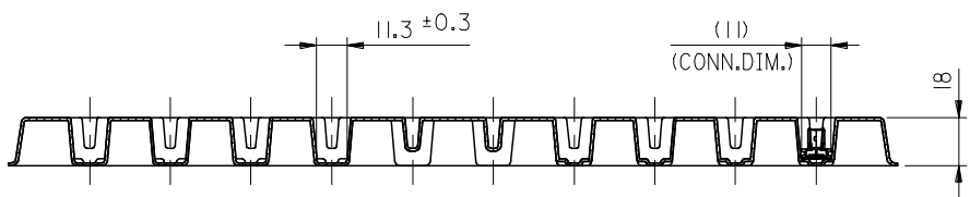
SECT. X-X
