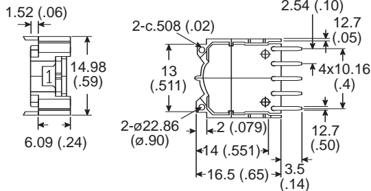
Mounting Terminals
