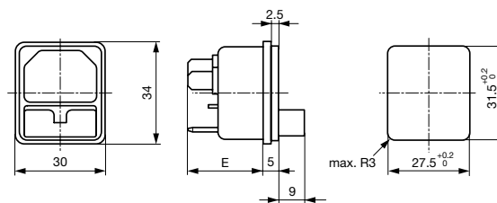
Snap-in mounting type 6220
