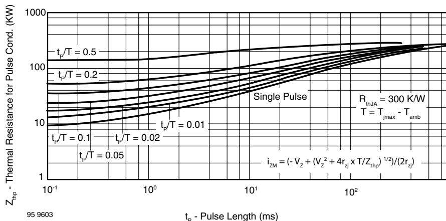
Figure 10. Thermal Response
