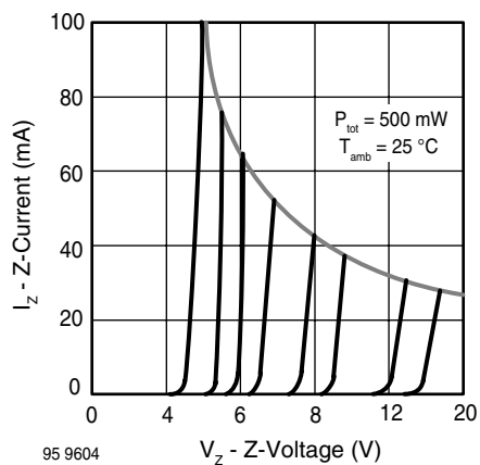
95 9604 Figure 7. Z-Current vs. Z-Voltage
