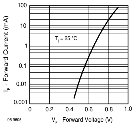
95 9605 Figure 6. Forward Current vs. Forward Voltage
